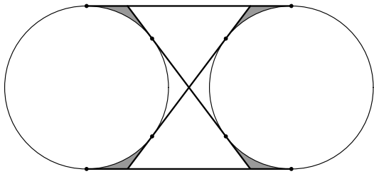
Figure 3: This figure shows two round circles forming an unlink L in the plane. The convex hull of L is bounded by a stadium curve. Its first hull h_1(L) , however, consists only of the hulls of the two components along with the four shaded triangular regions. These are bounded by the four lines tangent to both circles.
