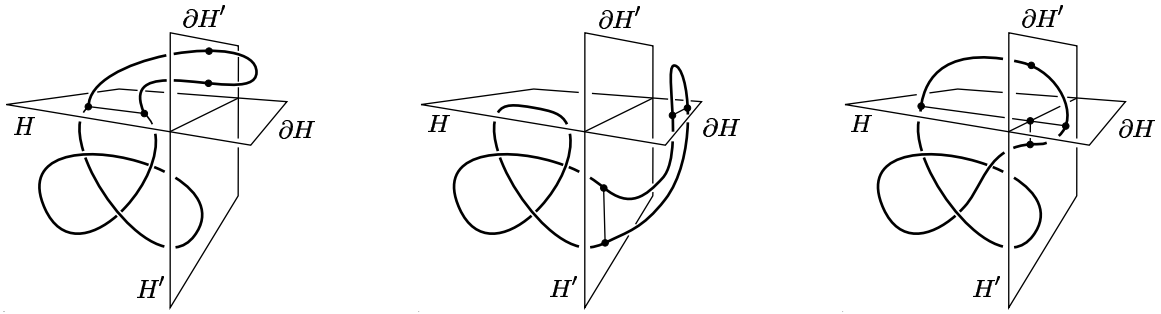
Figure 2: This figure shows the three cases of interest in the proof of Lemma 3. On the left, we see the case where both intersections of K with \partial H' occur outside H . In the center, we see the case where both intersections of K with \partial H' occur inside H . On the right, we see the case where K intersects \partial H' once inside and once outside H . In each figure, the segments in \partial H and \partial H' replacing unknotted subarcs of K when K is clipped to these planes are drawn in lightly. The half-space H is below the horizontal plane \partial H , while the half-space H' is to the left of the vertical plane \partial H' .
