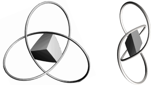
Figure 1: This figure shows the second hull of a trefoil knot, the shaded region in the center of the knot, from two perspectives. Every plane which intersects second hull must cut the knot at least four times. The trefoil shown here is a polygonal approximation to the critical point—and presumed minimizer—for the Möbius-invariant knot energy of Freedman, He and Wang [FHW94]. The region shown is an accurate computation of the second hull of this polygonal knot, produced by John Foreman. The sharp edges remind us that second hulls, like convex hulls, need not be as smooth as the curves which generate them.
