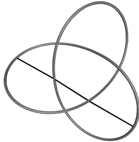
Figure 6: This figure shows an essential quadrisequant of a particular configuration of a trefoil knot. By Lemma 9, the mid-segment of this quadrisequant is contained within the second hull of K . In fact, this quadrisequant is alternating as well, so our earlier argument gives an alternate proof that the mid-segment is in the second hull of K . Since this is the same configuration of trefoil knot used in Figure 1, it is interesting to compare this picture with the image of the entire second hull.
